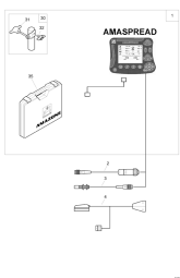
ETB-001409, Pakiet terminala AMASPREAD
