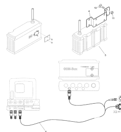
ETB-001420, Modem GSM CCI
