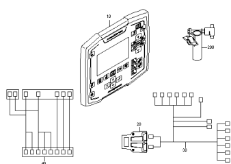
ETB-0000005449, Terminal Amasread 2
