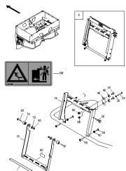
ETB-001374, Drabina S
