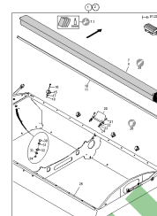
ETB-001426, Plandeka zwijana S i L
